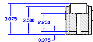
CROSS SECTION VIEW A-A
